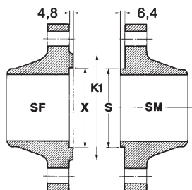
INCAMERATURA SEMPLICE STRETTA SMALL MALE AND FEMALE
