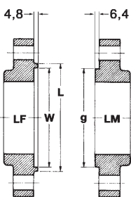
INCAMERATURA SEMPLICE LARGA LARGE MALE AND FEMALE
