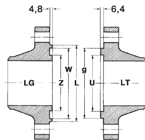
INCAMERATURA DOPPIA LARGA LARGE TONGUE AND GROOVE
